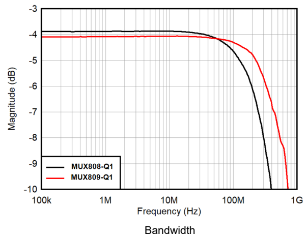
Figure 6-16. Insertion Loss vs Frequency
