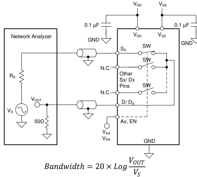
Figure 7-11. Bandwidth Measurement Setup
