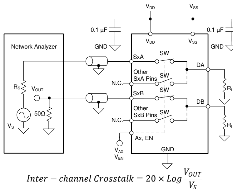
Figure 7-10. Inter-channel Crosstalk Measurement Setup
