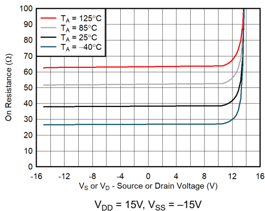
Figure 6-5. On-Resistance vs Source or Drain Voltage
