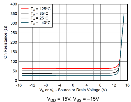
Figure 6-6. On-Resistance vs Source or Drain Voltage
