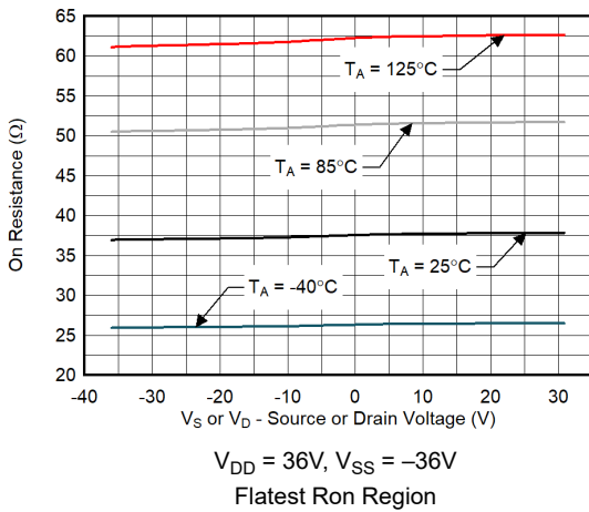
Figure 6-1. On-Resistance vs Source or Drain Voltage
