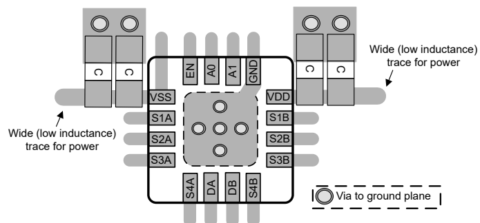
Figure 9-7. MUX809-Q1 QFN Layout Example
