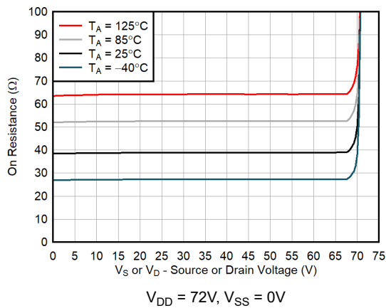
Figure 6-7. On-Resistance vs Source or Drain Voltage
