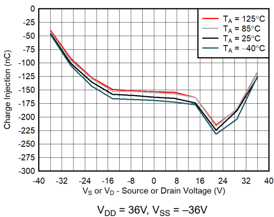
Figure 6-11. Charge Injection vs Source Voltage
