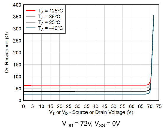
Figure 6-8. On-Resistance vs Source or Drain Voltage
