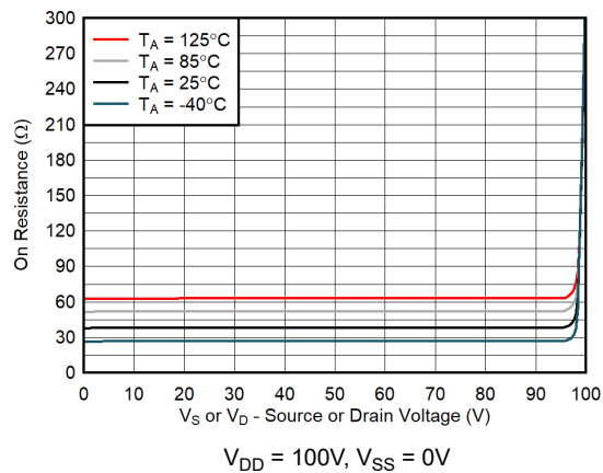
Figure 6-10. On-Resistance vs Source or Drain Voltage
