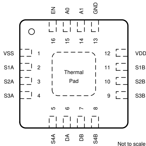
Figure 5-3. PW Package, 16-Pin TSSOP (Top View) Figure 5-4. RUM Package, 16-Pin WQFN (Top View)
