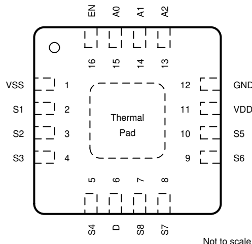
Figure 5-1. PW Package, 16-Pin TSSOP (Top View) Figure 5-2. RUM Package 16-Pin WQFN (Top View)
