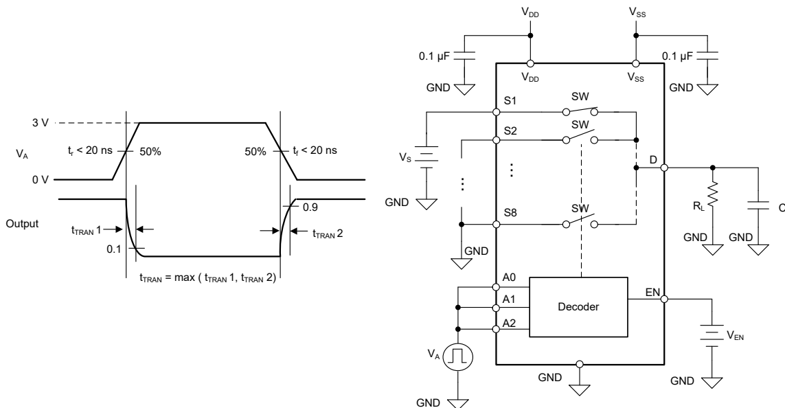
Figure 7-6. Transition Time Measurement Setup
