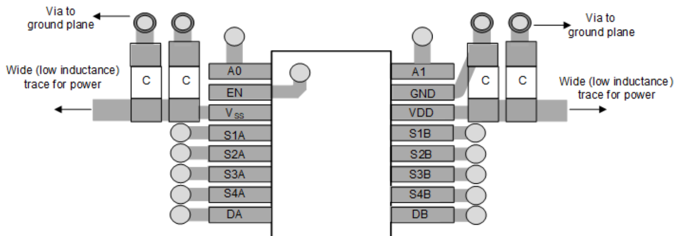
Figure 9-6. MUX809-Q1 TSSOP Layout Example
