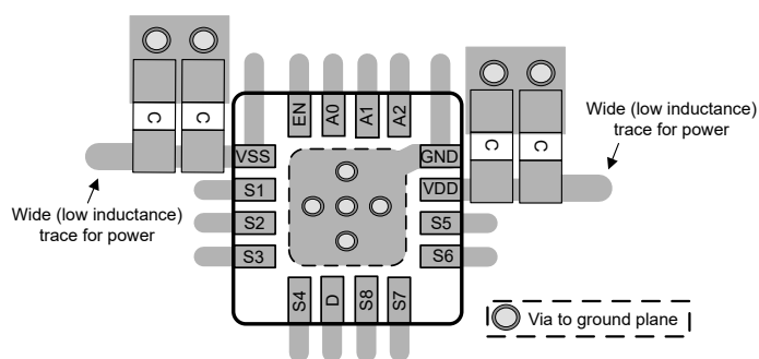
Figure 9-5. MUX808-Q1 QFN Layout Example
