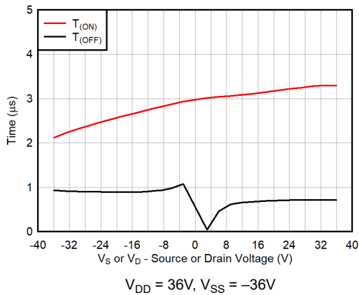
Figure 6-13. Turn-On and Turn-Off Times vs Source Voltage
