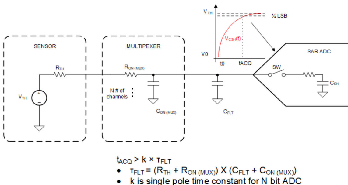
Figure 9-2. Driving SAR ADC
