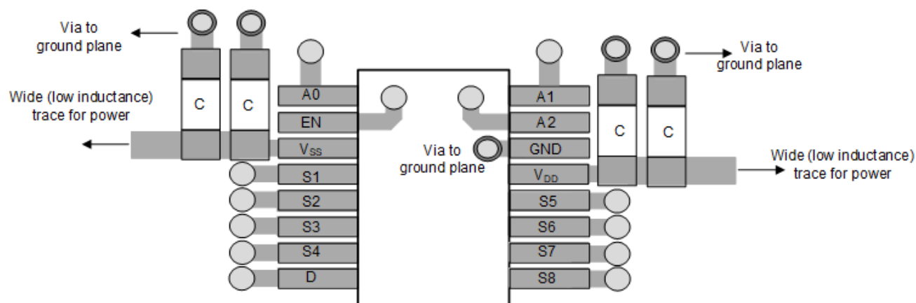
Figure 9-4. MUX808-Q1 TSSOP Layout Example
