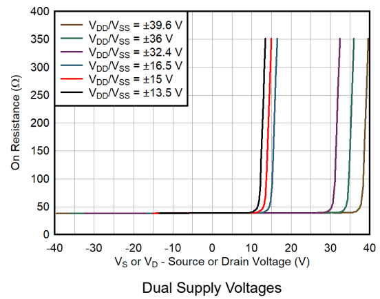
Figure 6-4. On-Resistance vs Source or Drain Voltage
