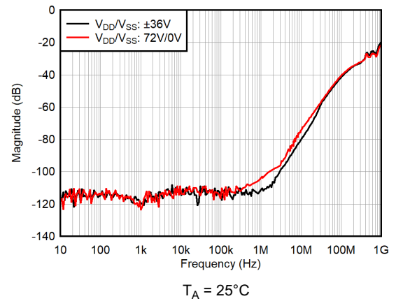
Figure 6-14. Off Isolation vs Frequency
