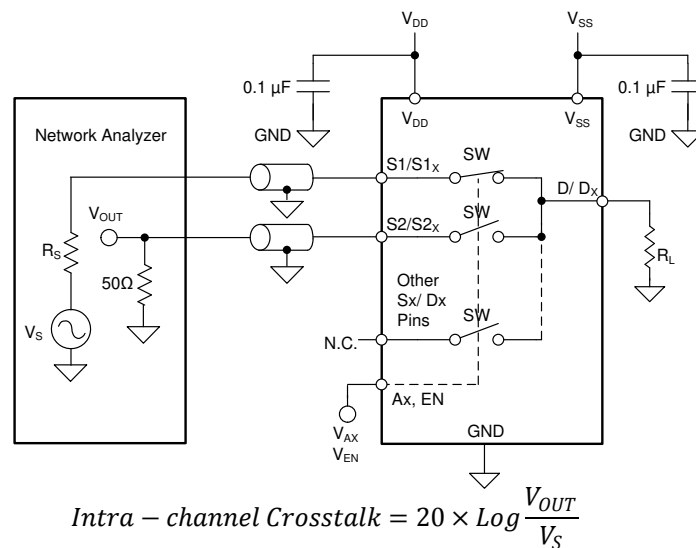
Figure 7-9. Intra-channel Crosstalk Measurement Setup
