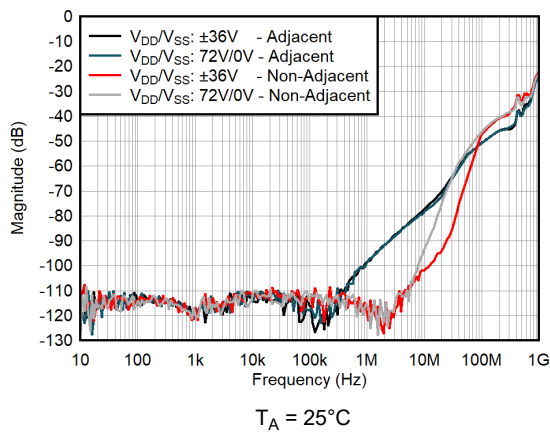
Figure 6-15. Crosstalk vs Frequency
