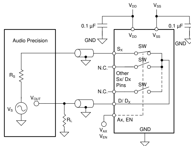
Figure 7-12. THD+N Measurement Setup
