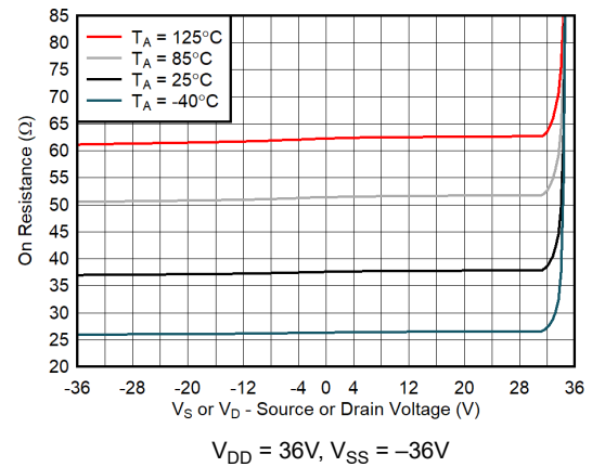
Figure 6-2. On-Resistance vs Source or Drain Voltage
