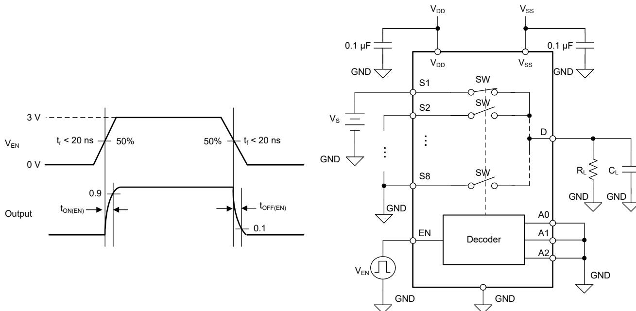
Figure 7-5. Enable Delay Measurement Setup
