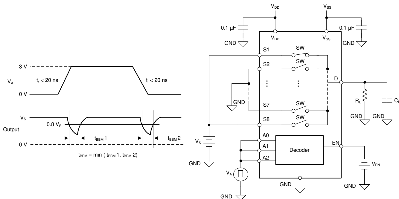
Figure 7-4. Break-Before-Make Delay Measurement Setup
