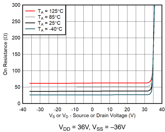
Figure 6-3. On-Resistance vs Source or Drain Voltage
