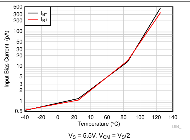
Figure 6-14. I_B vs Temperature
