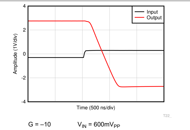
Figure 6-58. Overload Recovery
