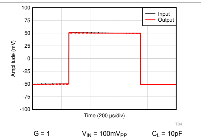
Figure 6-60. Small-Signal Step Response
