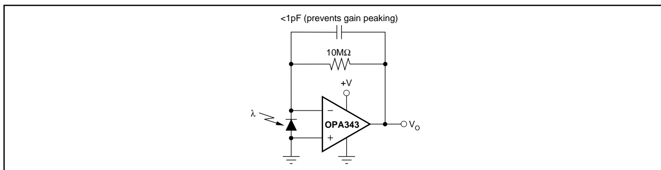
FIGURE 8. Transimpedance Amplifier.
