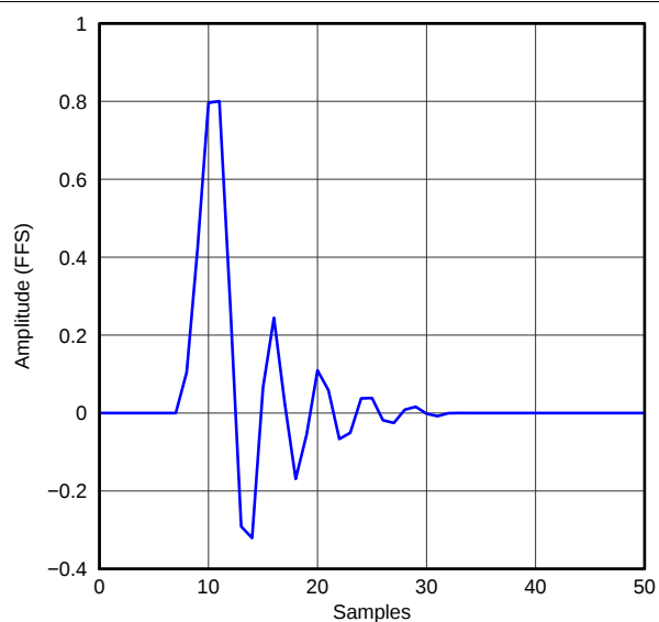
Figure 46. Asymmetric FIR x2 Interpolation Filter Impulse Response, Quad Rate
