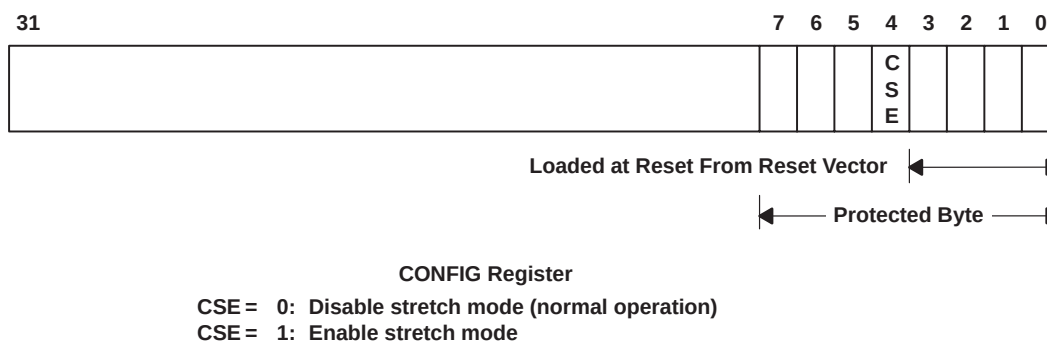
Figure 4. Stretch-Mode Enable
