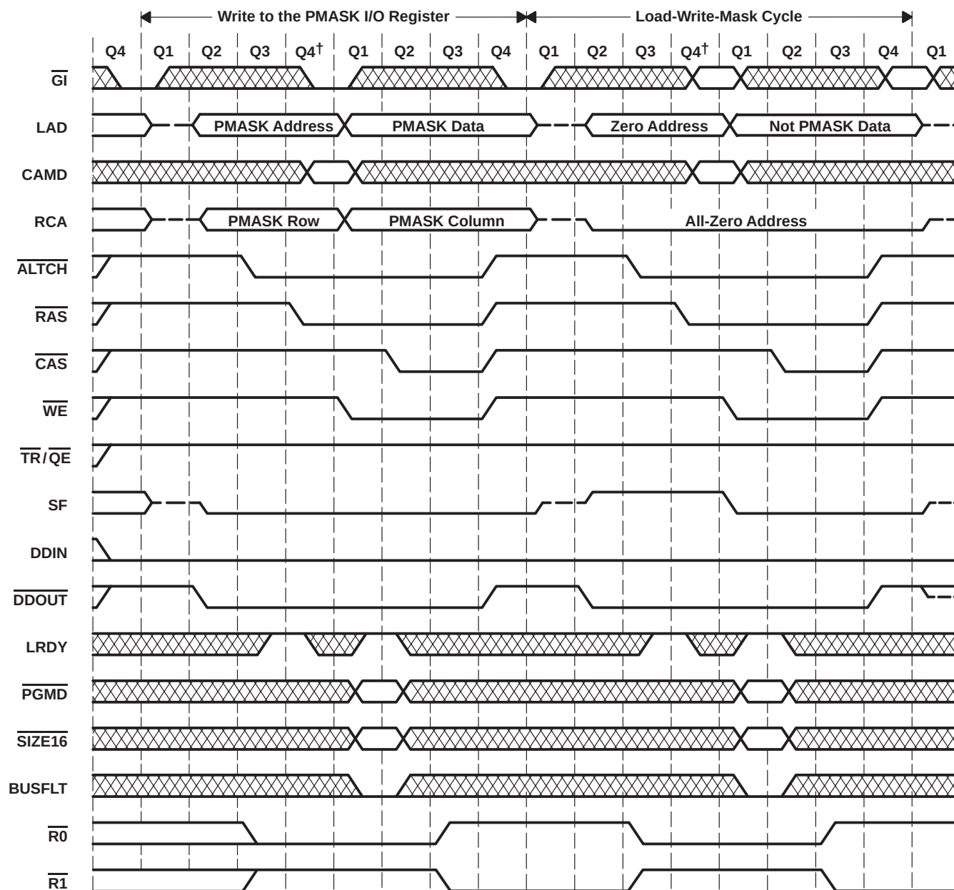
Figure 16. Load-Write-Mask Cycle
