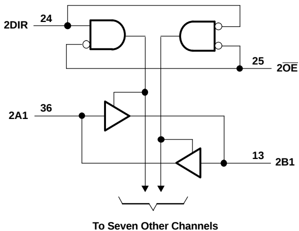
LOGIC DIAGRAM (POSITIVE LOGIC)
