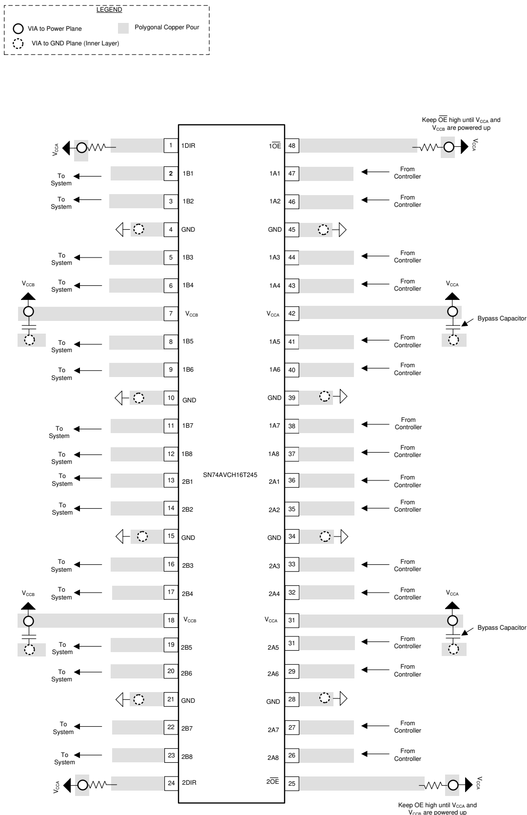
Figure 9-3. Recommended Layout Example
