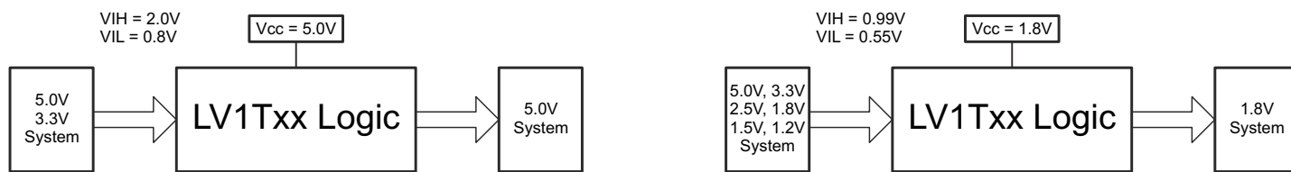
Figure 7-2. LVxT Up and Down Translation Example
