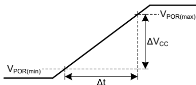
Figure 7-3. Supply ( V_{CC} ) Ramp Characteristics for Known Power-Up State
