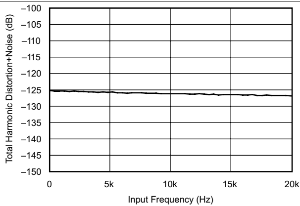
Figure 47. THD+N vs Input Frequency With 0 dBFS (96 kHz:48 kHz)
