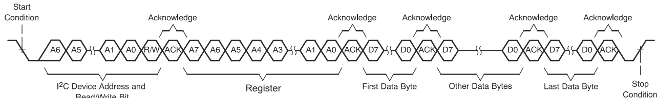
Figure 6-9. I 2 C Multiple-Byte Write Transfer
