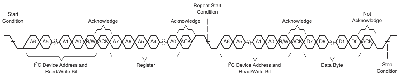
Figure 6-10. I 2 C Single-Byte Read Transfer
