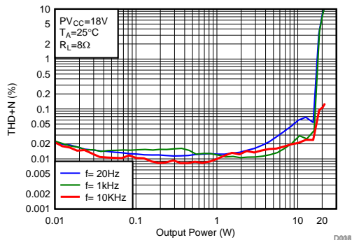
Figure 15. THD+N vs Output Power-BTL
