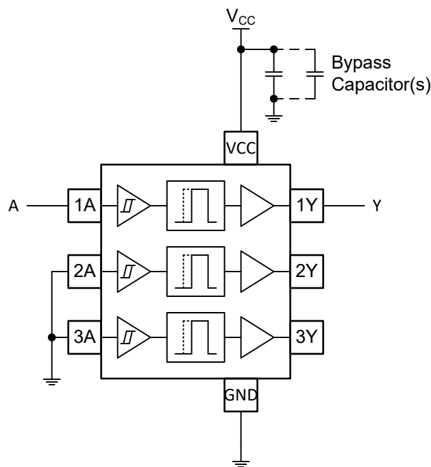
Figure 8-1. Rising Edge Delay Schematic Using the TDEL3G511
