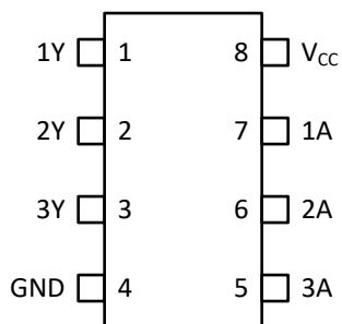
Figure 4-1. TDEL3G511 DRL Package (Top View)
