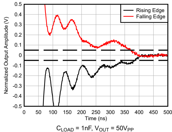
Figure 5-21. Large-Signal Settling Time
