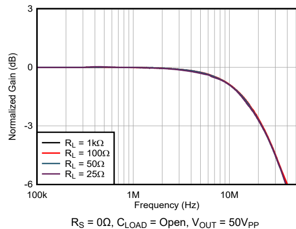
Figure 5-14. Large Signal Bandwidth vs Resistive Load
