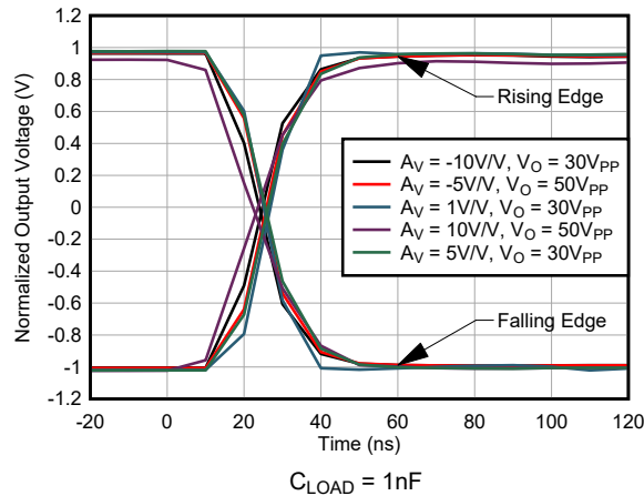
Figure 5-19. Large-Signal Step Response vs Gain
