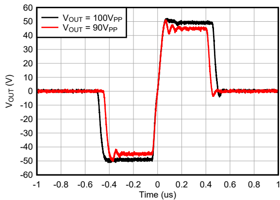
Figure 7-8. THS3470 Bootstrap Step Response ( V_{OUT} = 1\text{kV}/\mu\text{s} , R_L = 100\Omega , C_L = 1\text{nF} )
