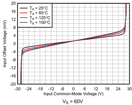
Figure 5-43. Input Offset vs Input Common-Mode
