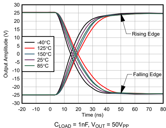
Figure 5-17. Large-Signal Step Response vs Temperature
