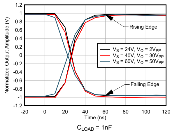
Figure 5-18. Large-Signal Step Response vs Supply Voltage
