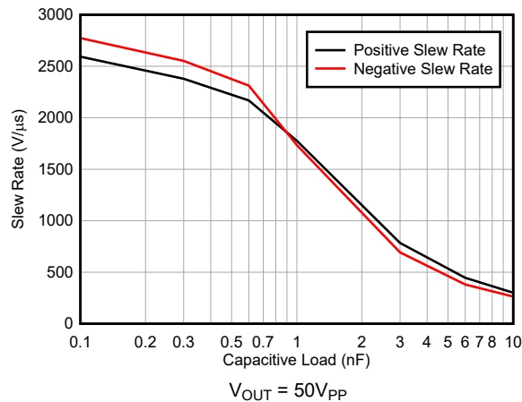
Figure 5-15. Slew Rate vs Capacitive Load
