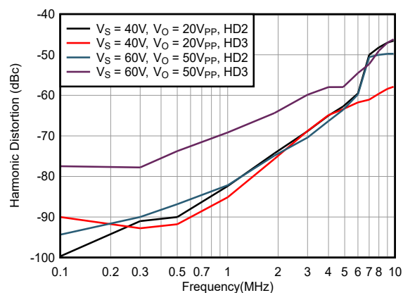
Harmonic Distortion vs Frequency ( R_{LOAD} = 100\Omega )
