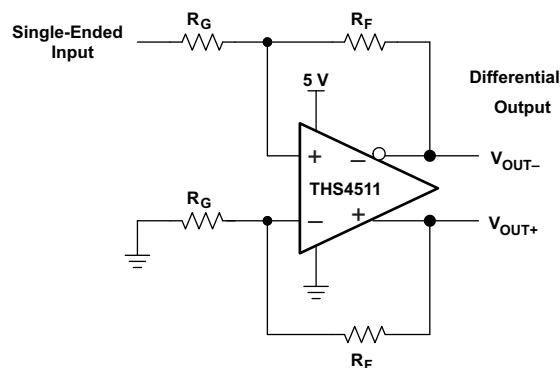
Figure 36. Single-Ended Input to Differential Output Amplifier
