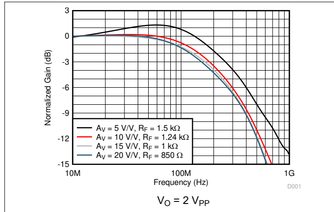
Figure 5-1. Small-Signal Frequency Response
