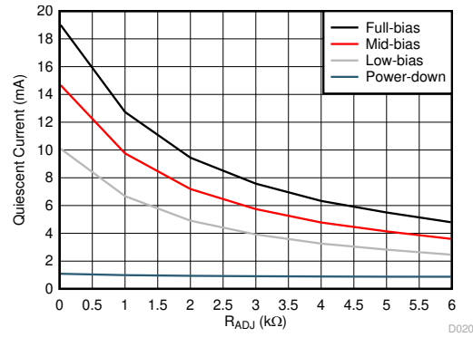
Figure 5-32. Quiescent Current vs R_{ADJ}
