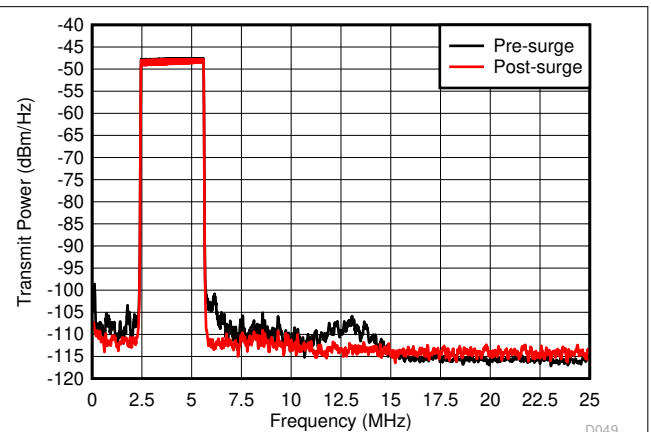
Figure 6-9. China SGCC HPLC Band1 Pre-Surge and Post-Surge
