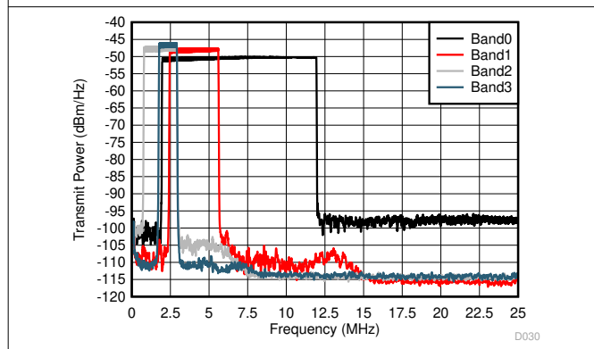
SGCC HPLC profiles, crest factor = 5 V/V, see the Broadband PLC Line Driving section for more details.
