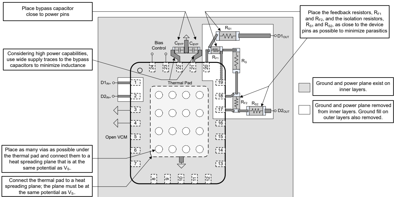
Figure 7-6. Layout Recommendations
