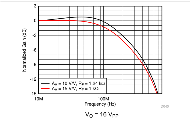
Figure 5-2. Large-Signal Frequency Response
