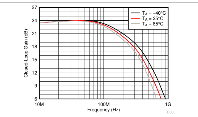
Figure 5-2. Large-Signal Frequency Response
