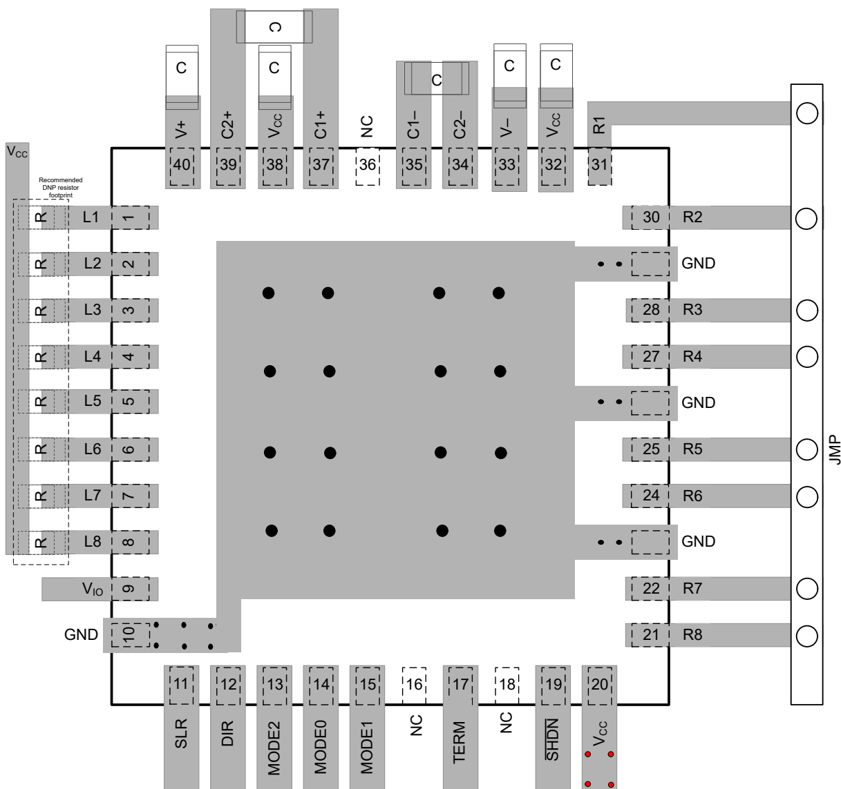
Figure 8-14. Layout Example
