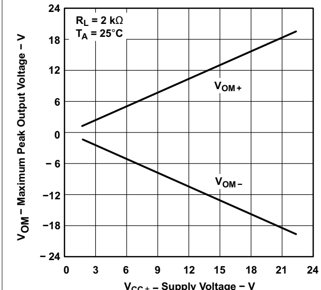
Figure 5-7. Maximum Peak Output Voltage vs Supply Voltage
