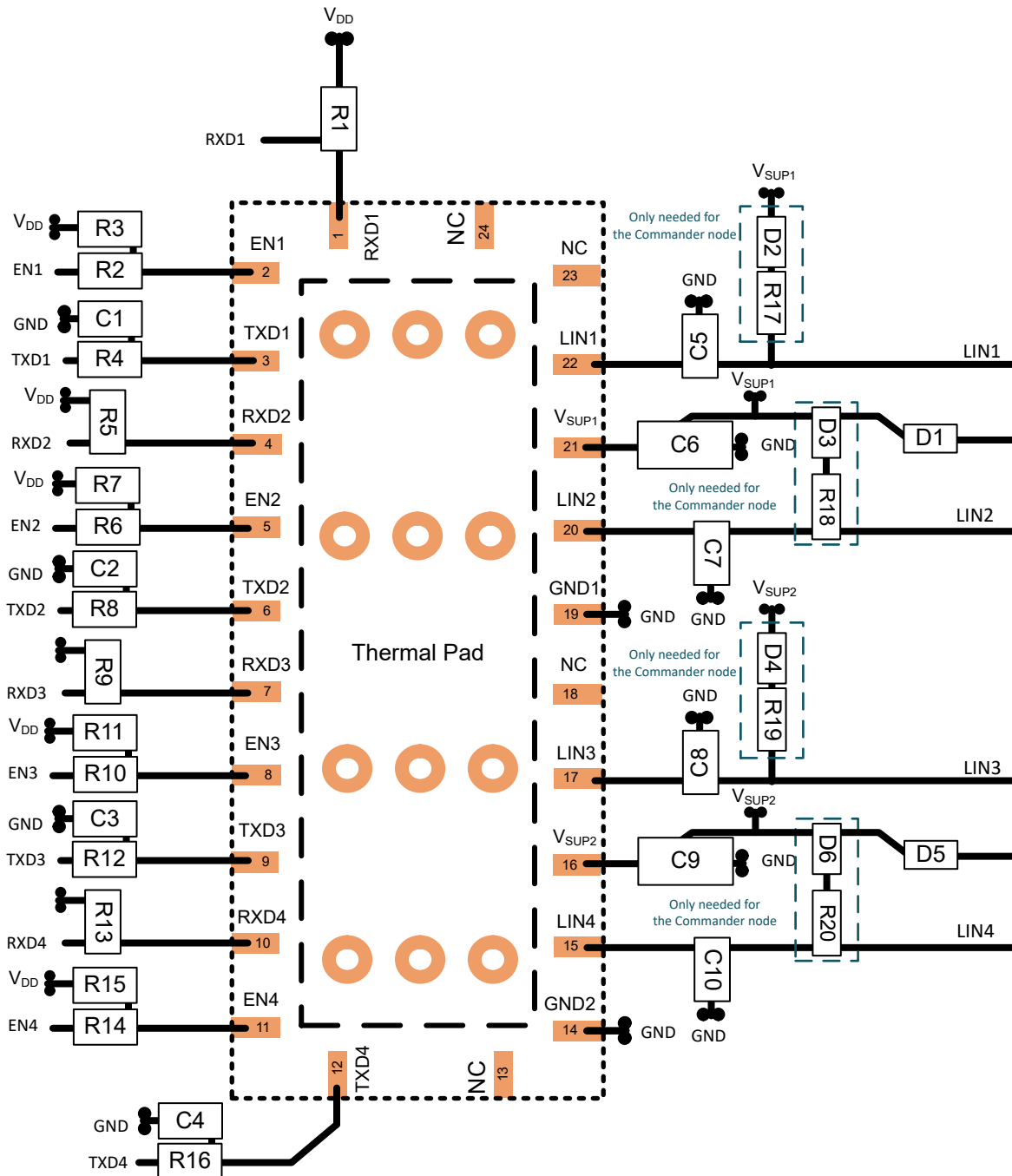
Figure 8-4. Layout Example
