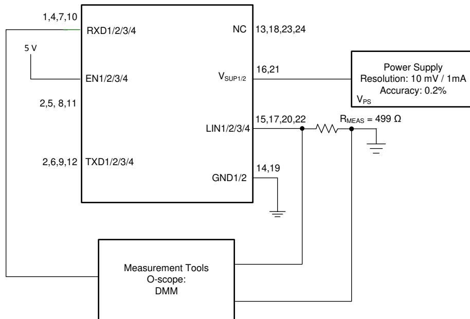
Figure 7-7. Test Circuit for I_{BUS\_PAS\_dom} ; TXD = Recessive State V_{BUS} = 0\text{ V}
