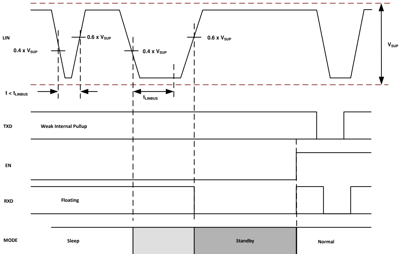
Figure 7-17. Wake Up Through LIN
