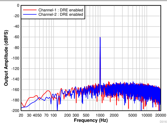
Figure 7-19. FFT With a -60-dB Input With DRE Enabled
