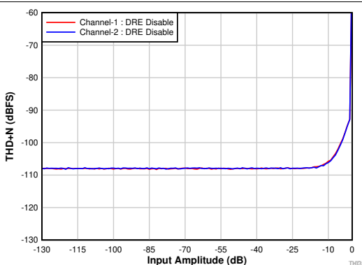
Figure 7-26. THD+N vs Input Amplitude With DRE Disabled
