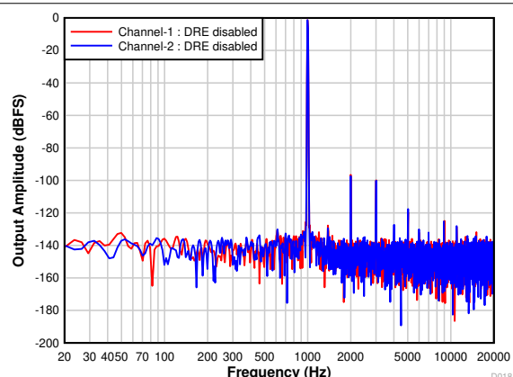
Figure 7-21. FFT With a -1-dB Input With DRE Disabled
