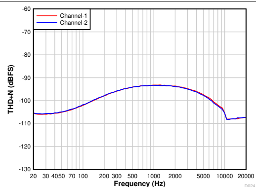
Figure 7-27. THD+N vs Input Frequency at -1-dBr Input With DRE Disabled
