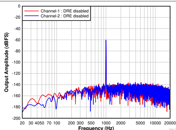
Figure 7-20. FFT With a -60-dB Input With DRE Disabled
