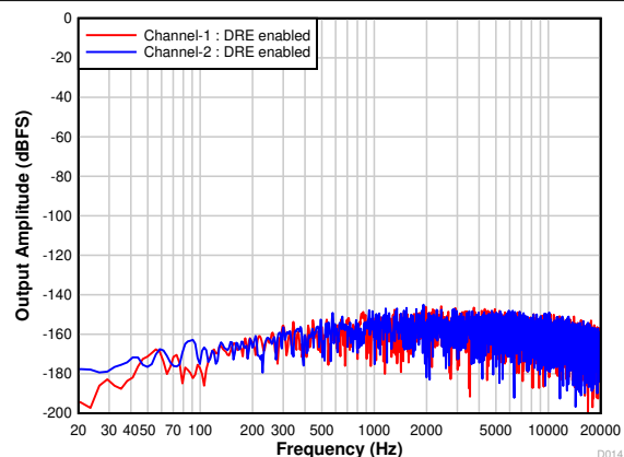
Figure 7-17. FFT With Idle Input With DRE Enabled
