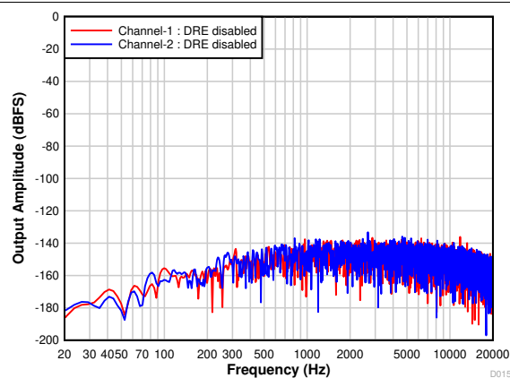
Figure 7-18. FFT With Idle Input With DRE Disabled
