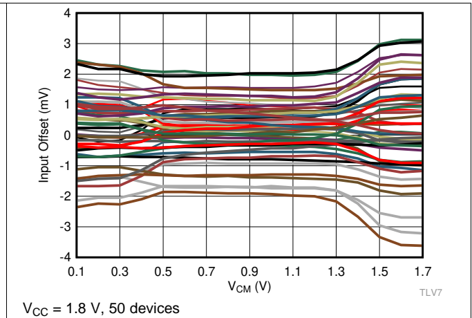
Figure 4. Input Offset Voltage vs. V_{CM}
