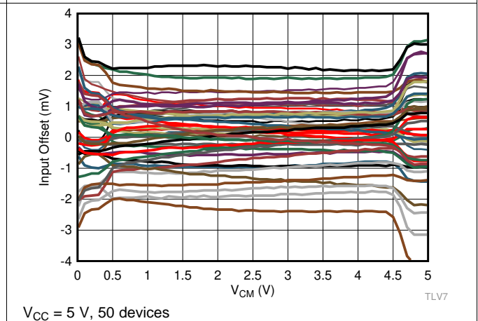
Figure 6. Input Offset Voltage vs. V_{CM}
