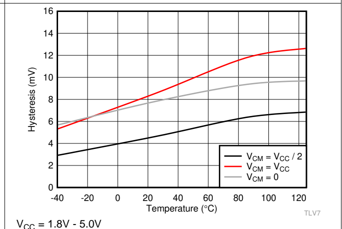
Figure 8. TLV70x1 Hysteresis vs. Temperature
