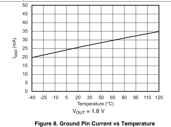
Figure 8. Ground Pin Current vs Temperature
