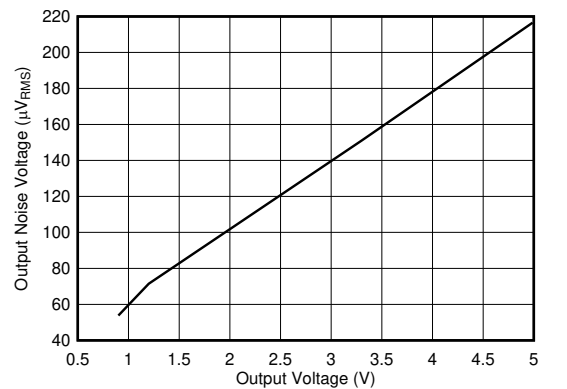
I_{OUT} = 500\text{mA} , C_{OUT} = 1\mu\text{F} , V_{RMS} BW = 10Hz to 100kHz Figure 5-6. Output Noise Voltage vs V_{OUT}
