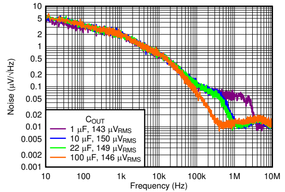
V_{OUT} = 3.3\text{V} , V_{RMS} BW = 10Hz to 100kHz Figure 5-4. Output Spectral Noise Density vs Frequency and C_{OUT}
