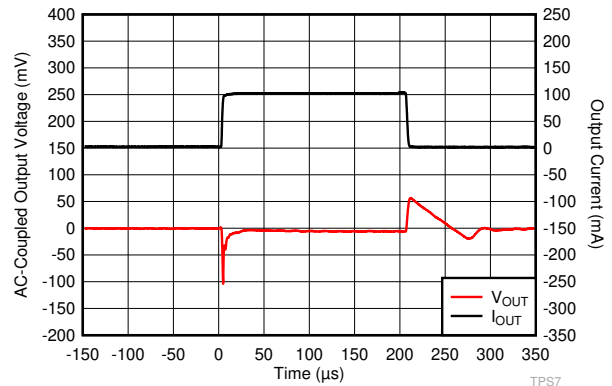
Figure 5-14. I_{OUT} Transient From 1mA to 100mA
