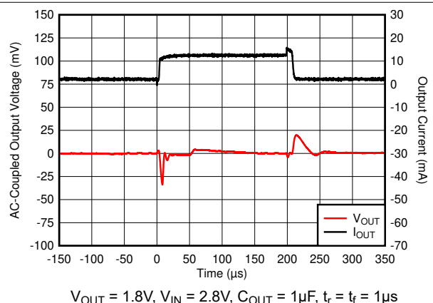
Figure 5-12. I_{OUT} Transient From 1\text{mA} to 10\text{mA}
