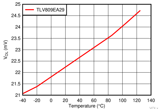
Figure 7-14. Low Voltage Output Verses Temperature for TLV809EA29, V_{DD} = 1.7\text{ V}
