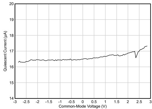
Figure 5-23. Quiescent Current vs Common-Mode
