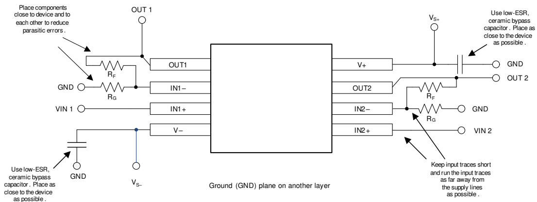
Figure 7-12. Layout Example
