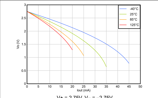
Figure 5-12. Output Voltage vs Output Current (Claw)
