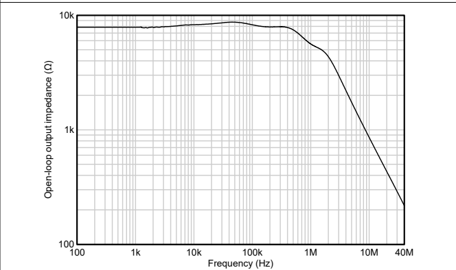
Figure 5-10. Open-Loop Output Impedance vs Frequency
