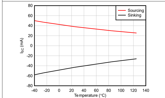
Figure 5-33. Short-Circuit Current vs Temperature
