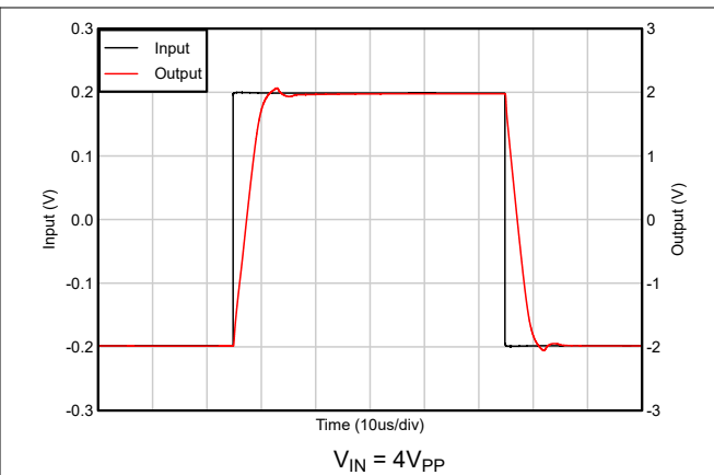
Figure 5-32. Large-Signal Step Response (TLV9042D)
