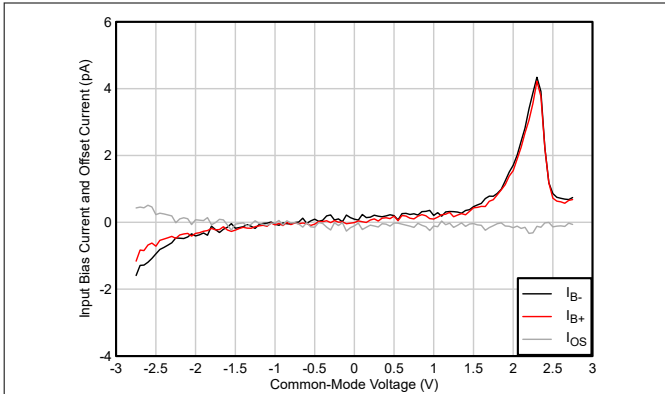
Figure 5-7. I_B and I_{OS} vs Common-Mode Voltage
