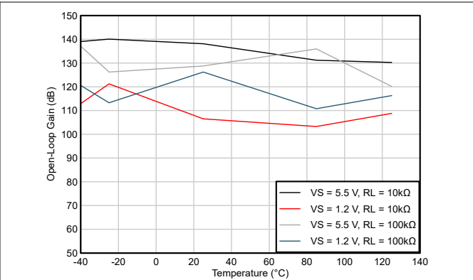
Figure 5-8. Open-Loop Gain vs Temperature
