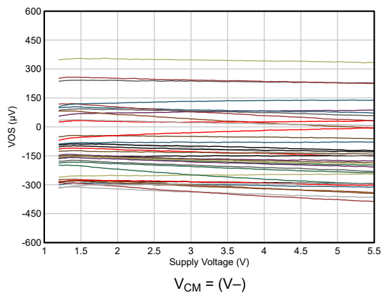
Figure 5-5. Offset Voltage vs Supply Voltage
