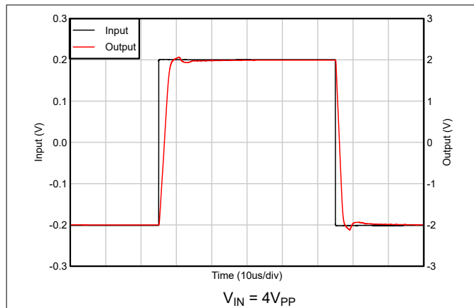
Figure 5-31. Large-Signal Step Response (TLV9041D)
