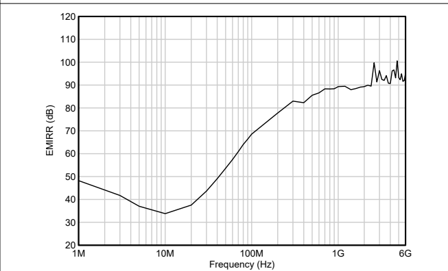
Figure 5-34. Electromagnetic Interference Rejection Ratio Referred to Noninverting Input (EMIRR+) vs Frequency
