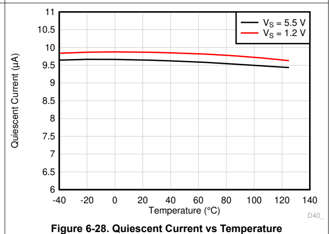
Figure 6-28. Quiescent Current vs Temperature
