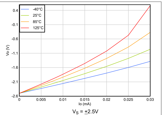
Figure 5-26. Output Voltage Swing vs Output Current (Sinking)
