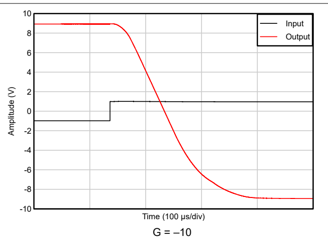
Figure 5-36. Overload Recovery (Positive)
