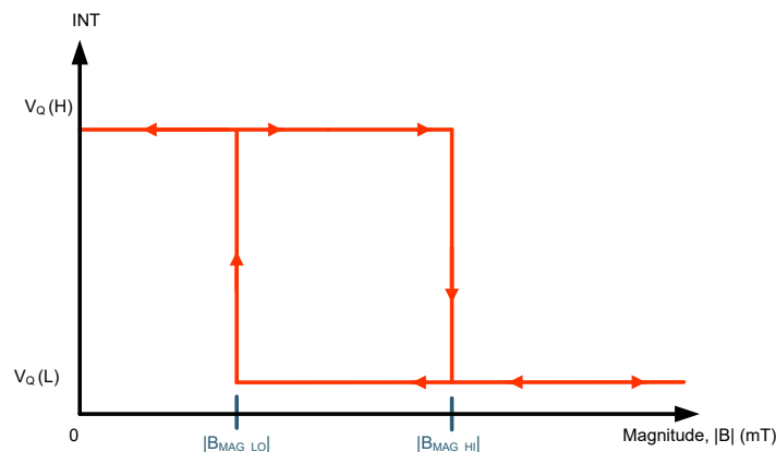
Figure 8-17. Magnitude Switch
