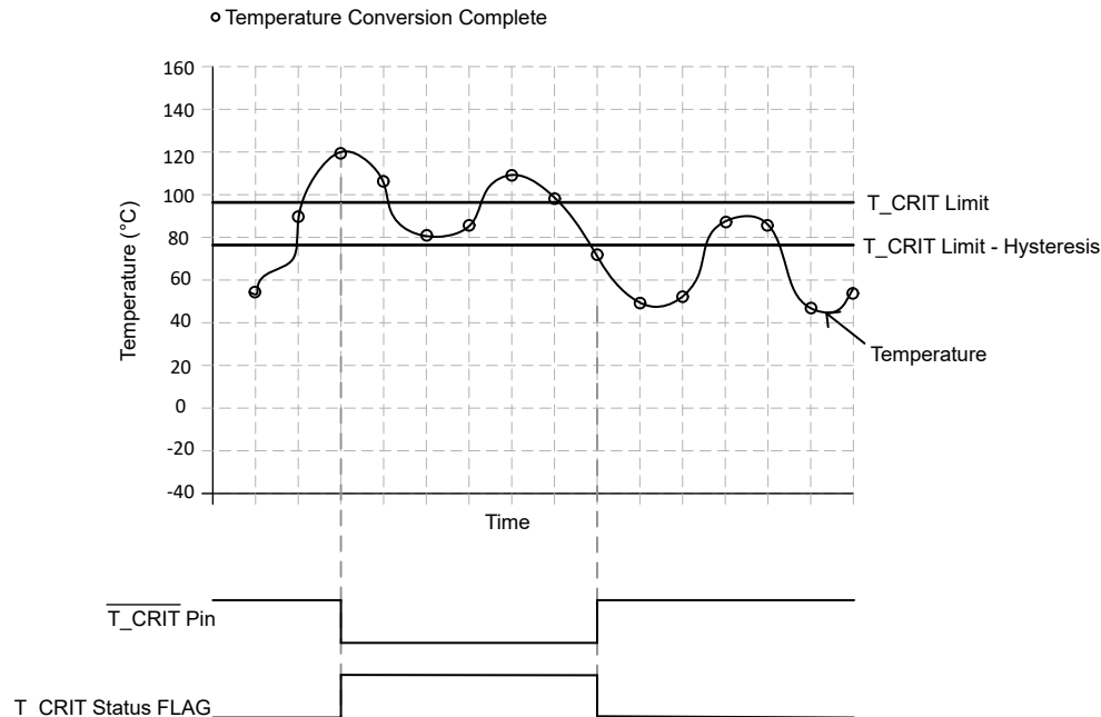
Figure 7-8. \overline{\text{T\_CRIT}} Output Timing Diagram-Comparator Mode
