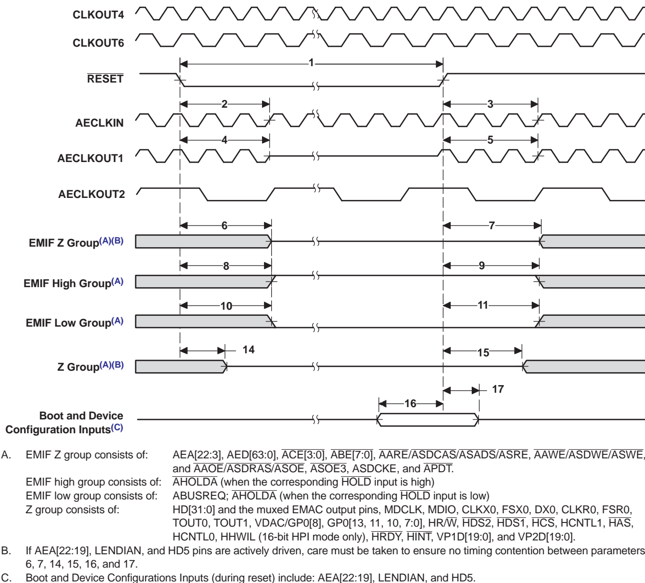
Figure 5-11. Reset Timing
