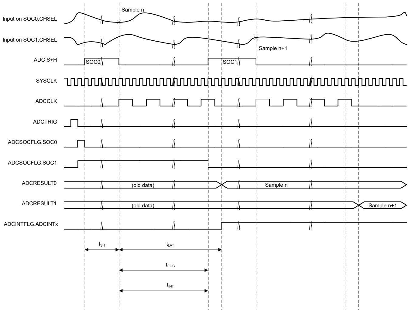
Figure 6-46. ADC Timings
