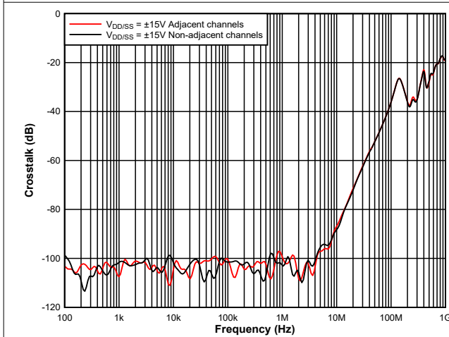
Figure 5-19. Crosstalk vs Frequency
