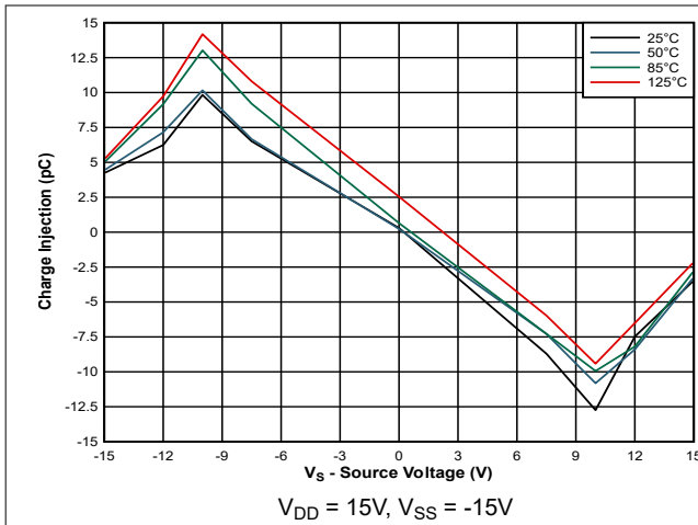
Figure 5-17. Charge Injection vs Source Voltage
