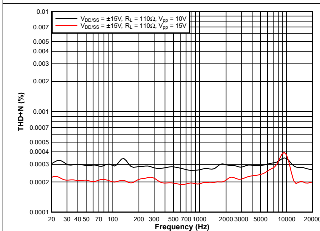
Figure 5-21. THD+N vs Frequency
