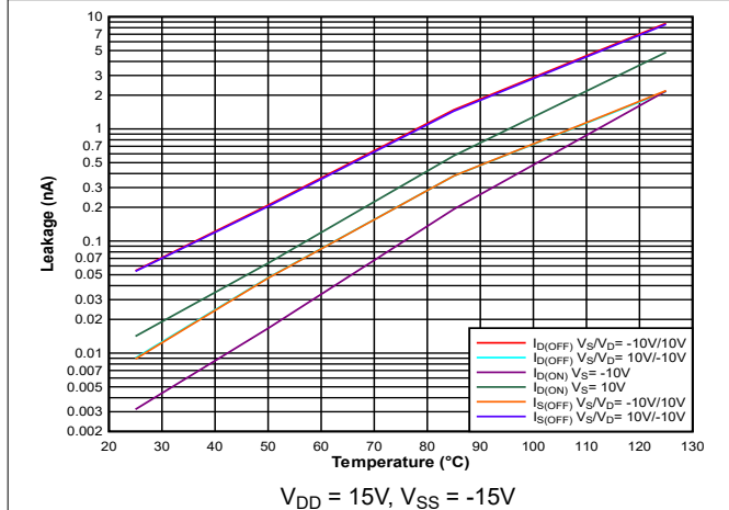
Figure 5-9. Leakage Current vs Temperature
