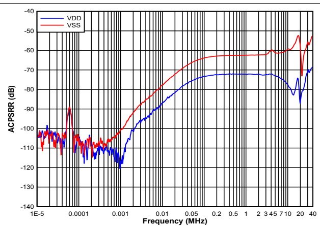
Figure 5-22. ACPSSR vs Frequency
