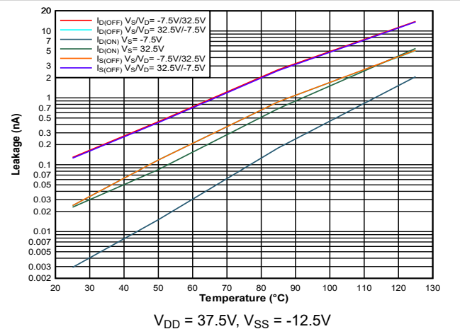
Figure 5-10. Leakage Current vs Temperature
