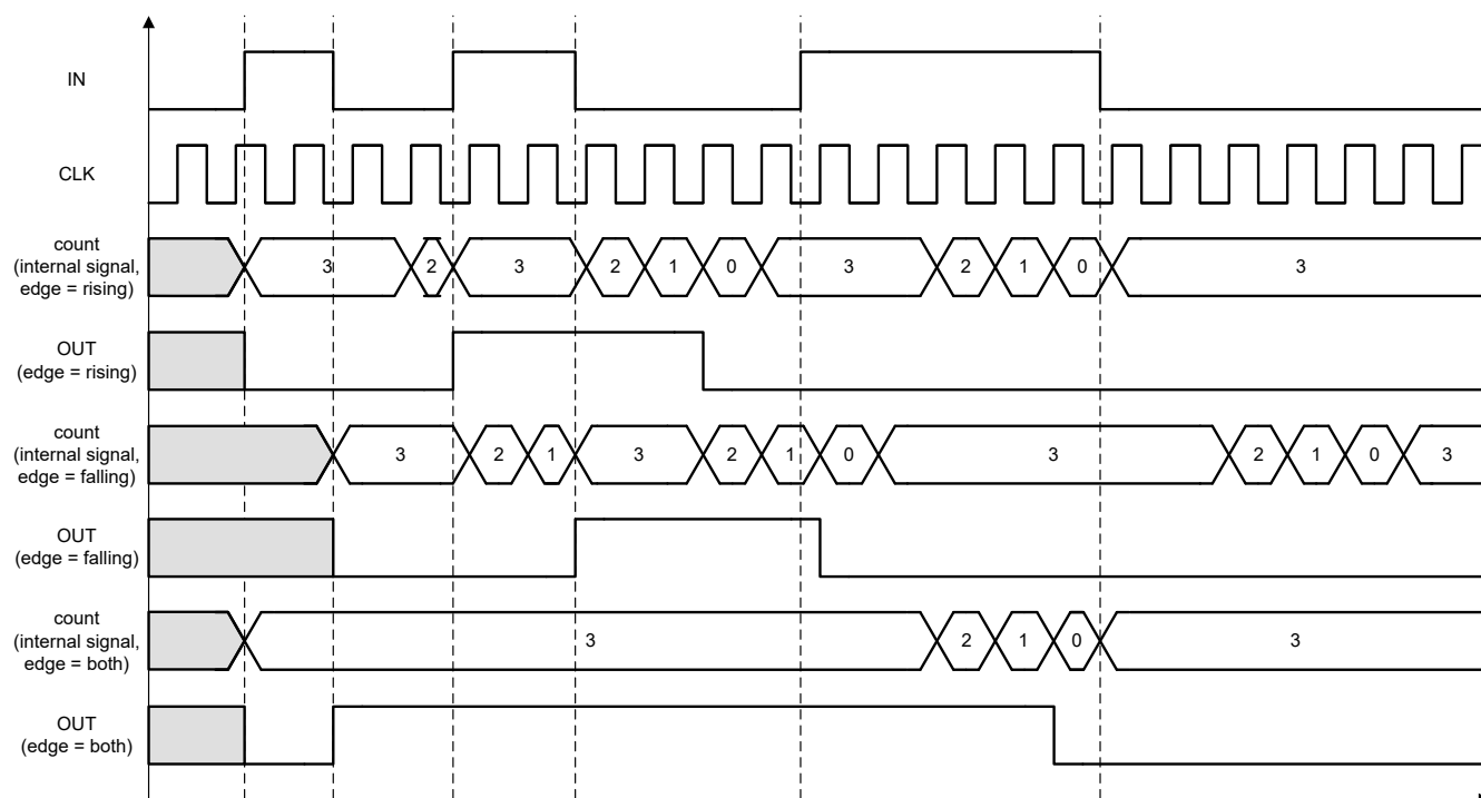
Figure 8-19. Frequency detector output timing example (DATA = 3)
