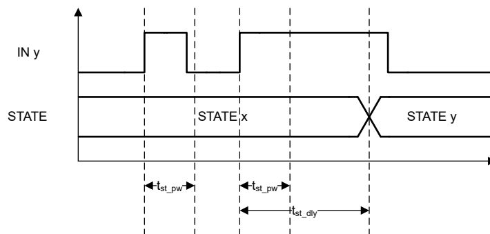
Figure 8-27. State transition trigger requirements timing example
