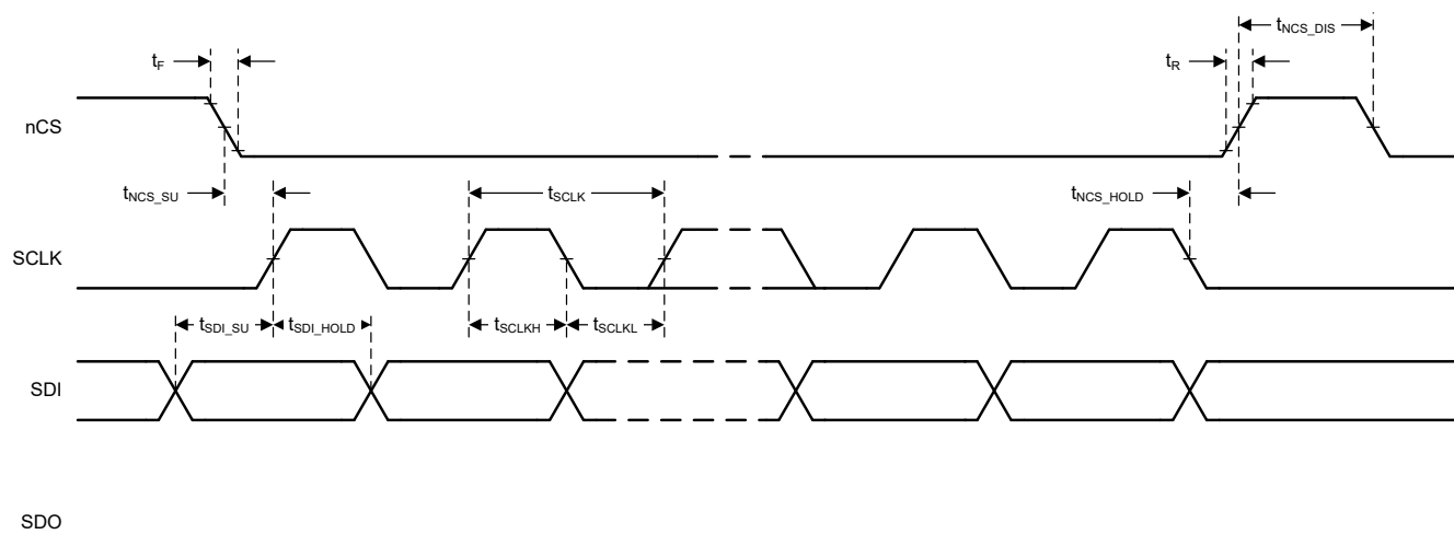
Figure 8-57. SPI Write Timing Diagram
