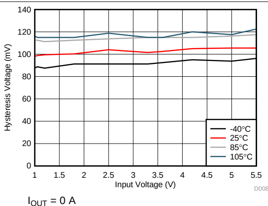
Figure 6. Hysteresis Voltage vs Input Voltage
