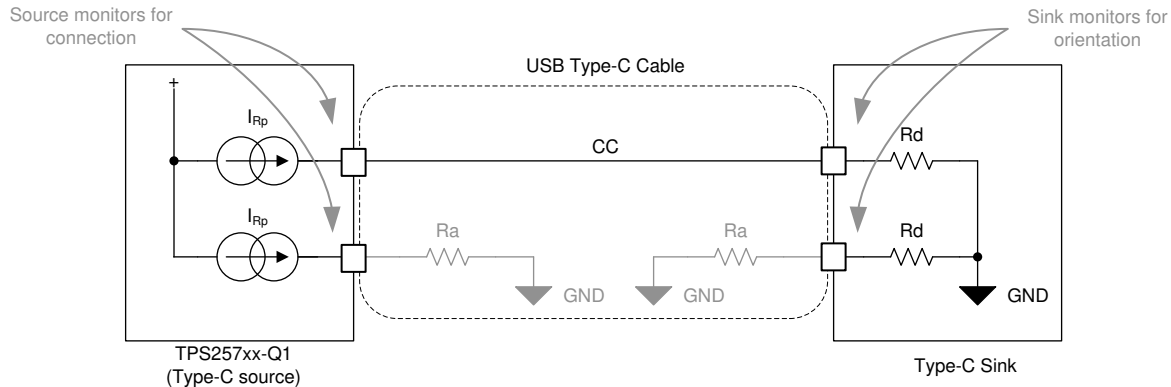
Figure 8-29. Type-C Cable
