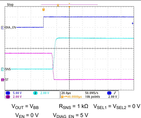
Figure 7-31. Open Load Detection Time ( t_{OL2} ) on Rising DIA\_EN
