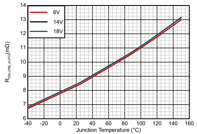
Figure 6-4. On resistance in AUTO_LPM ( R_{ON\_LPM\_AUTO} ) vs Temperature
