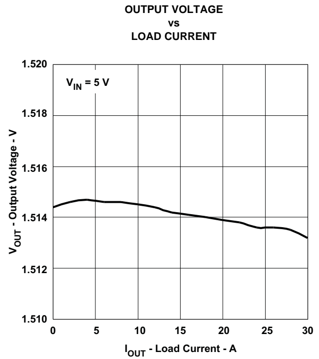
Figure 19. Load Regulation
