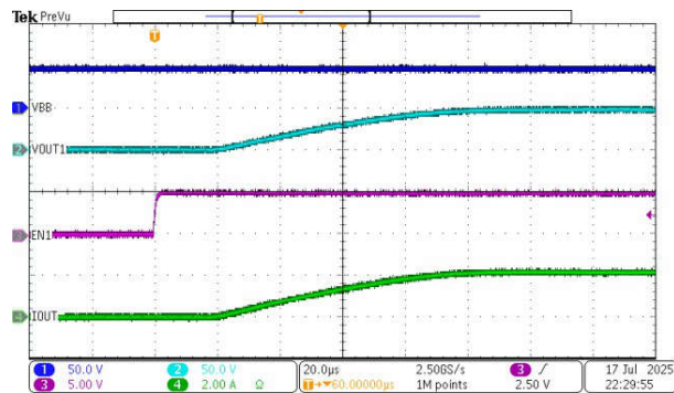
Figure 8-4. Turn-on with Resistive Load
