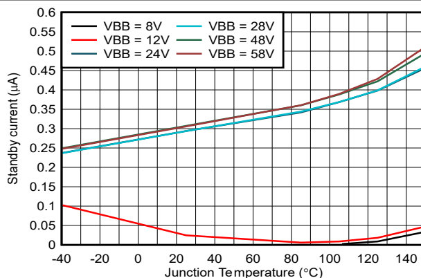
Figure 6-2. Standby Current
