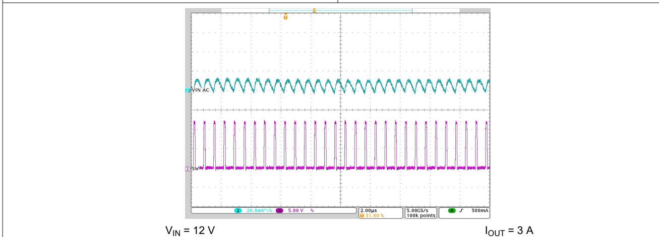
Figure 8-30. Input Ripple – 3-A Load
