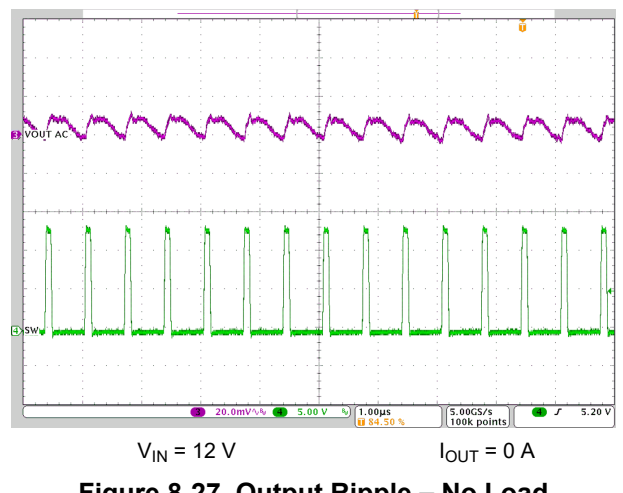
Figure 8-27. Output Ripple – No Load
