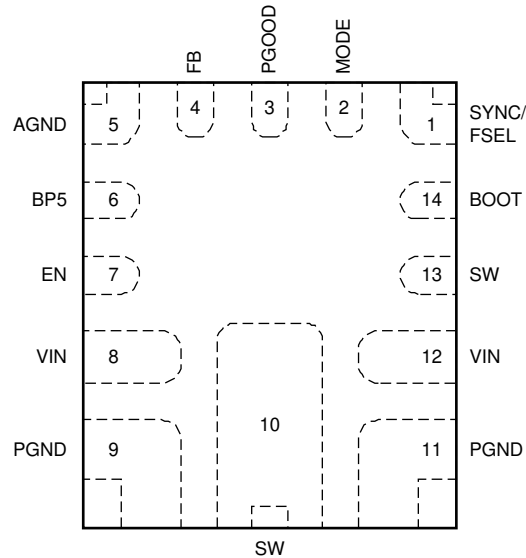
Figure 5-1. 14-Pin VQFN-HR RPY Package (Top View)
