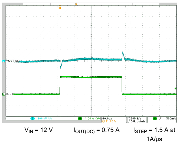
Figure 8-26. Load Transient
