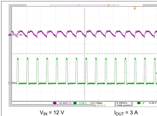
Figure 8-28. Output Ripple – 3-A Load
