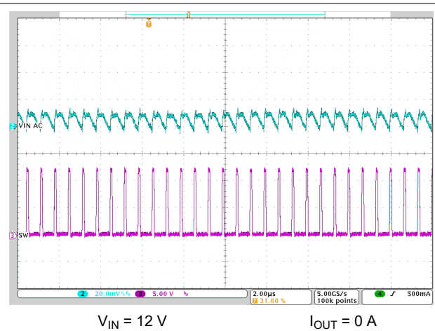
Figure 8-29. Input Ripple – No Load
