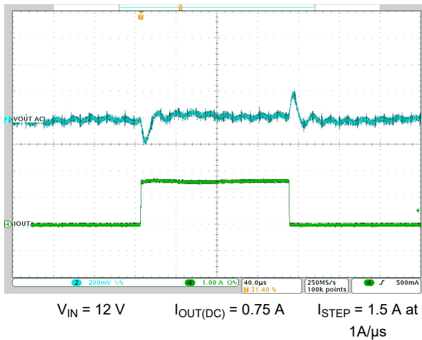
Figure 8-8. Load Transient
