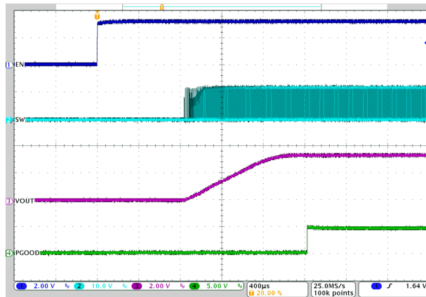
Figure 8-10. EN Startup – Measuring SW
