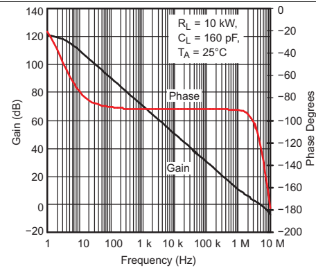
Figure 8. Error Amplifier vs Open Loop Response
