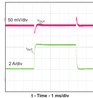
Figure 16. Transient Response
