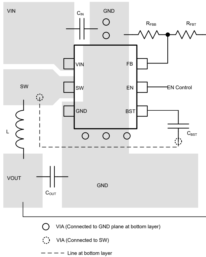
Figure 7-18. TPS56224xx Layout
