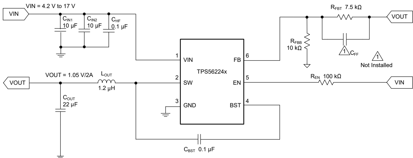
Figure 7-1. TPS56224xx 1.05V/2A Reference Design
