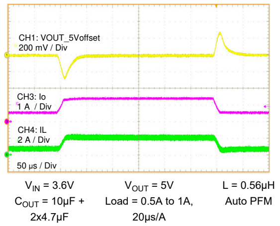
Figure 8-7. Load Transient
