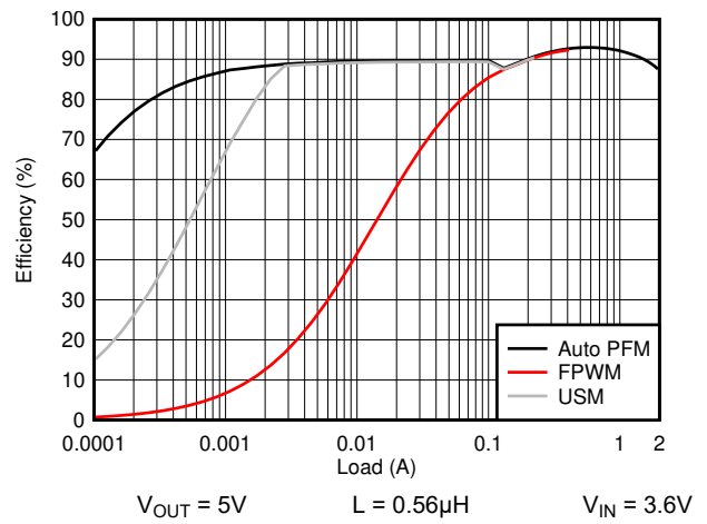
Figure 6-2. Efficiency vs Load
