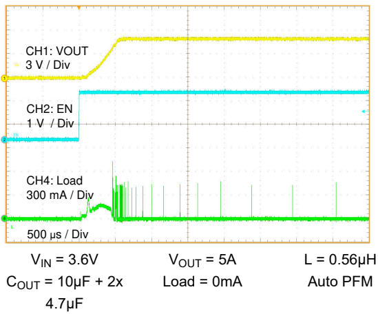
Figure 8-6. Start-up by EN
