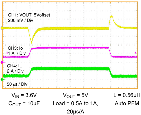
Figure 8-8. Load Transient with 10 \mu F C_{OUT}
