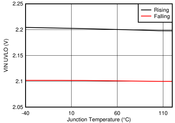
Figure 6-16. VIN UVLO vs Temperature
