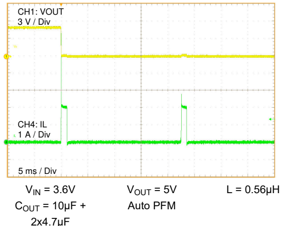
Figure 8-9. Short Output
