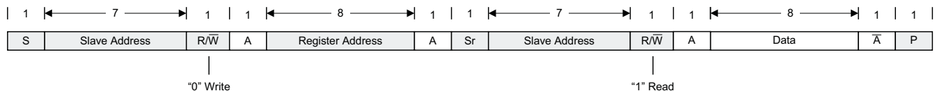
Figure 54. "Write" Data Transfer Format in Standard, Fast- and Fast-Plus Modes
