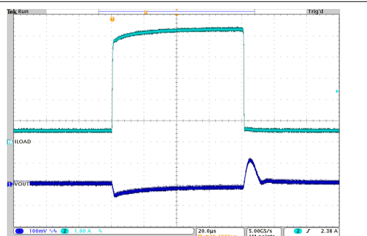
V_{OUT} = 0.6\text{ V} PWM T_A = 25^\circ\text{C} V_{IN} = 3.3\text{ V} I_{OUT} = 0.6\text{ A to } 5.4\text{ A to } 0.6\text{ A}
