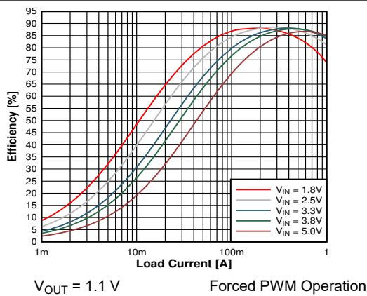
Figure 9-6. Efficiency, Inductor Comparison
