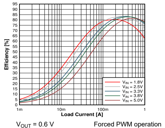
Figure 9-7. Efficiency
