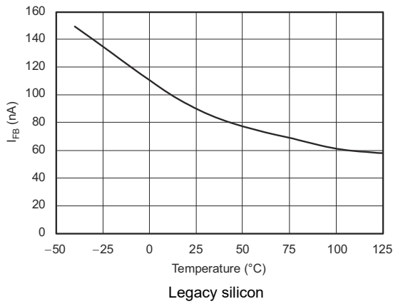
Figure 5-49. TPS73201 I_{FB} vs Temperature
