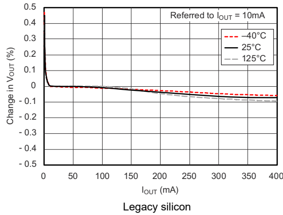
Figure 5-1. Load Regulation
