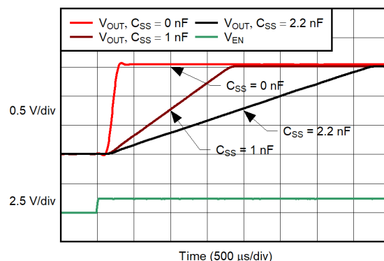
Turn-On Response
